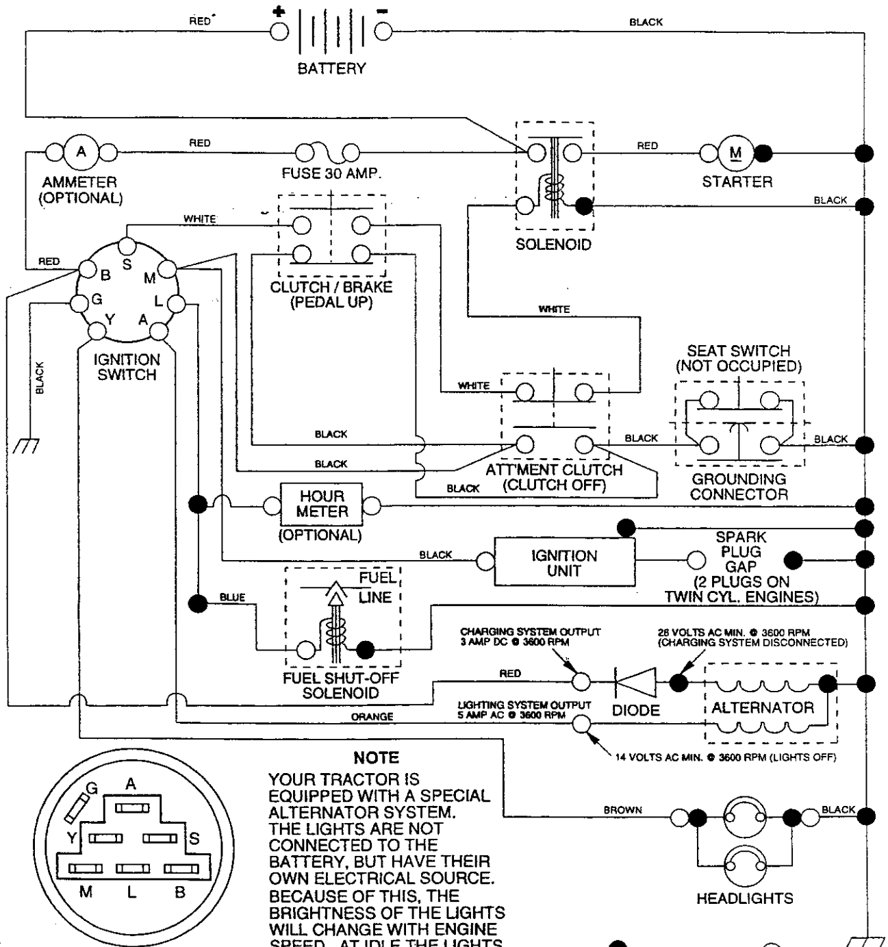
IGNITION SWITCH
