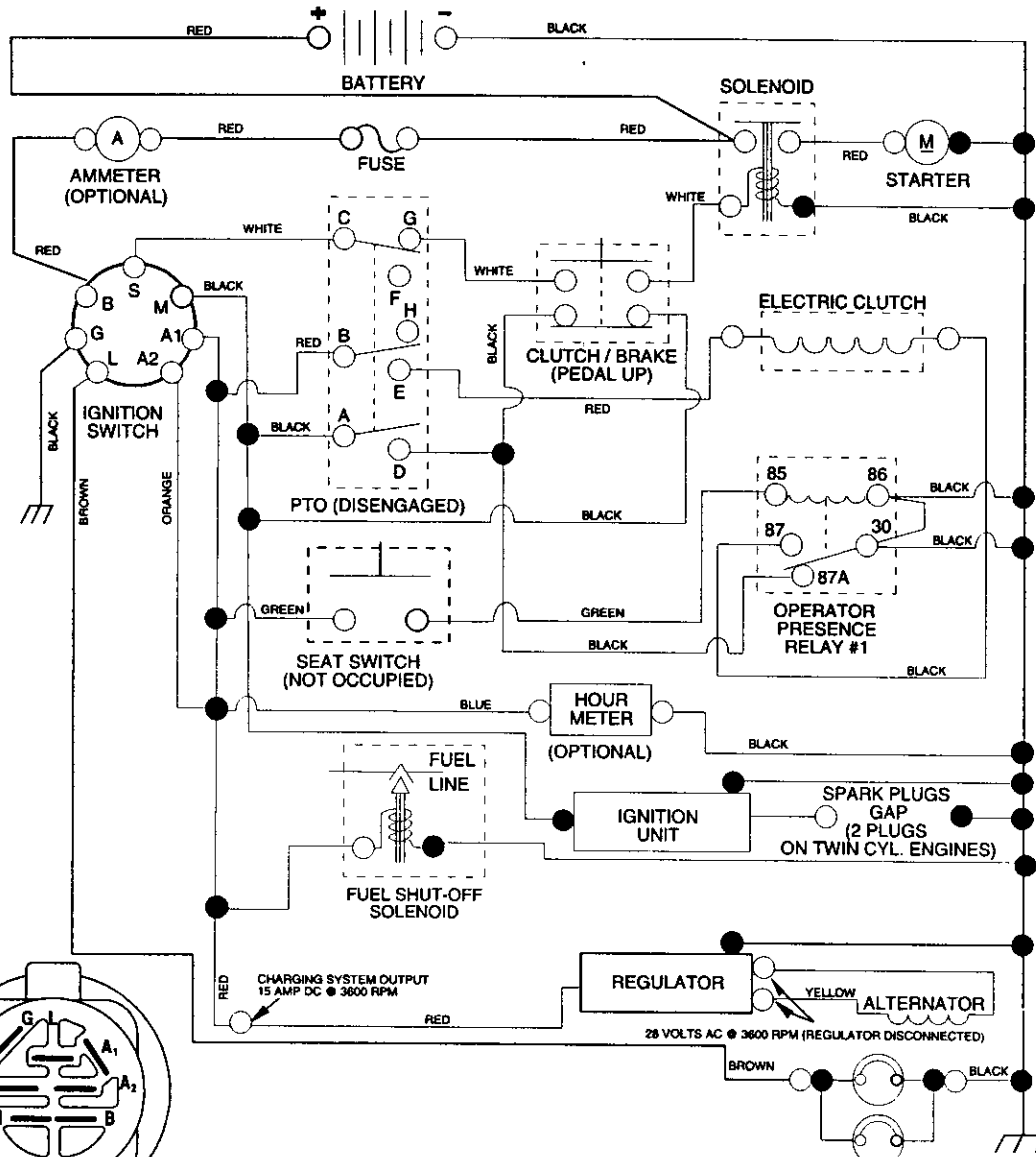
IGNITION SWITCH
