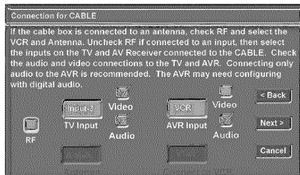
Figure 2. Connection menu.
