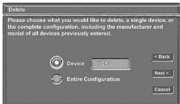
Figure 1. Delete menu.
