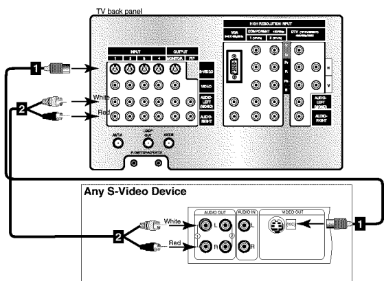
Figure 2. Connecting an S-Video Device.
