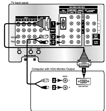
Figure 1. Connecting a computer with a VGA monitor output.
