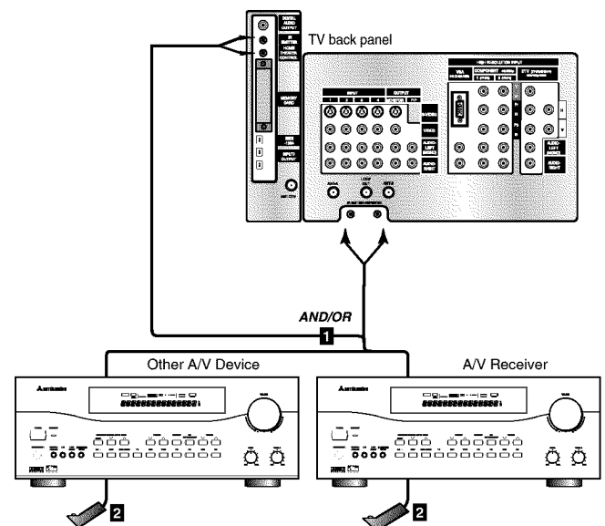
Figure 2. Connecting the IR Home Theater Control and/or Repeater.
