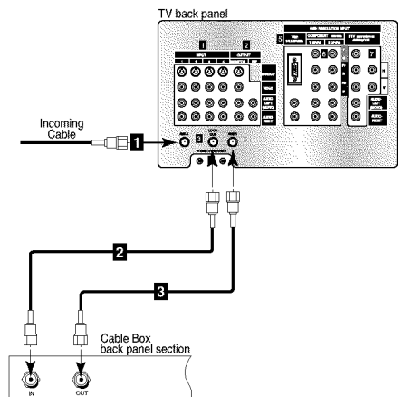
Figure 3. Connecting the cable box.
