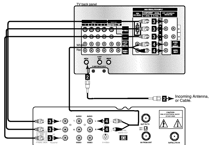
Figure 2. Connecting the DTV receiver with component video connections.
