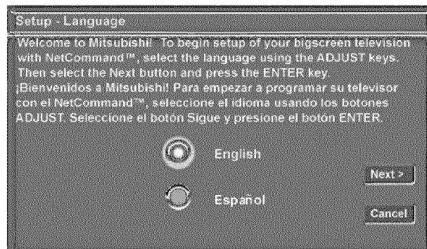
Figure 1. Setup-Language menu.
