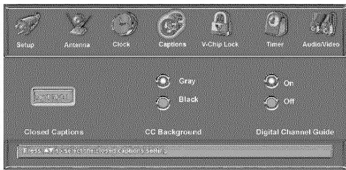
Figure 1. Captions menu
