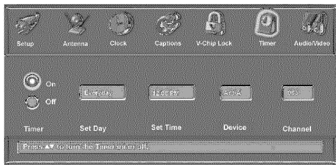
Figure 1. Timer menu
