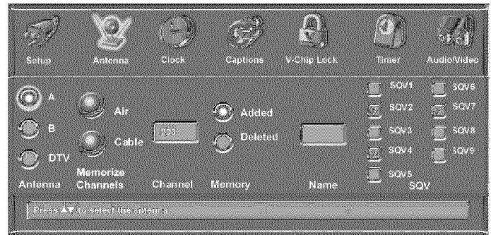
Figure 1. Antenna menu
