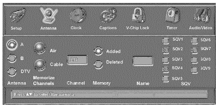
Figure 2. Antenna menu
