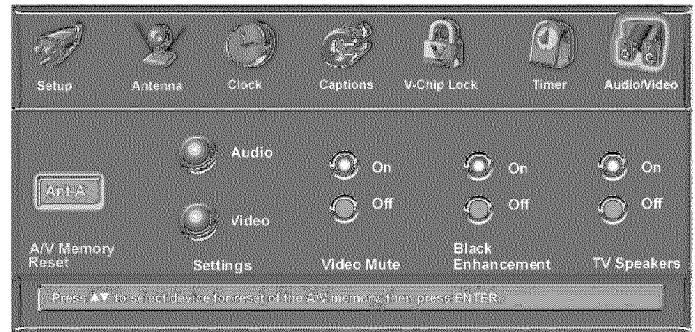
Figure 1. Audio/Video menu
