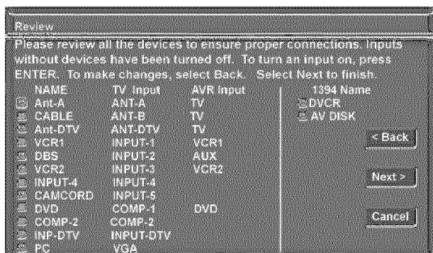
Figure 1. Review menu.
