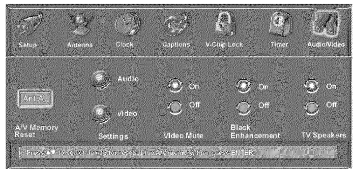
Figure 4. Audio/Video menu
