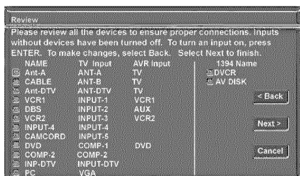
Figure 2. Review menu.
