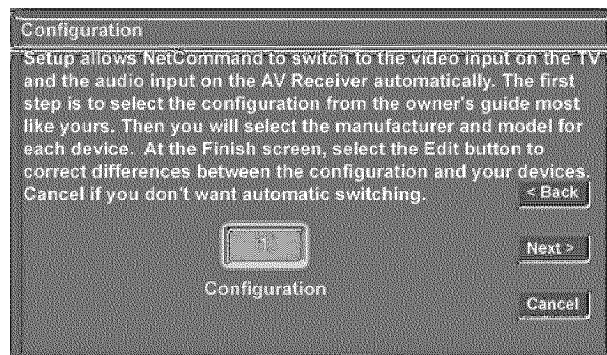
Figure 2. Configuration menu.
