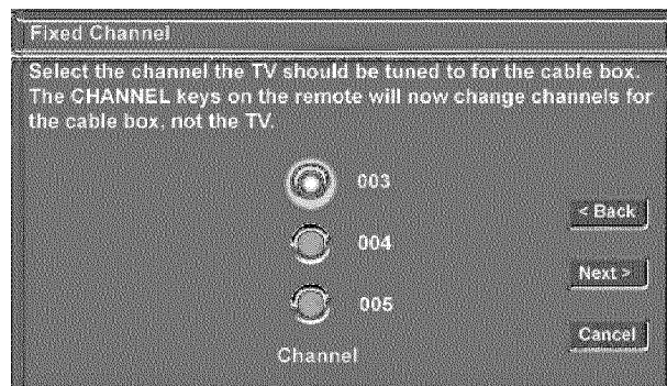
Figure 3. Channel menu.
