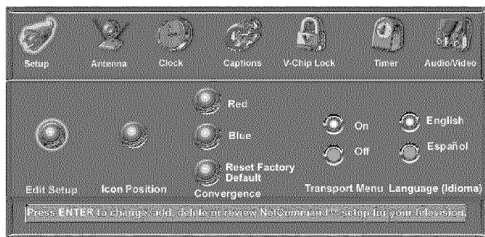
Figure 1. Setup menu
