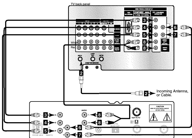
Figure 1. Connecting the DTV receiver with RGB video connections.
