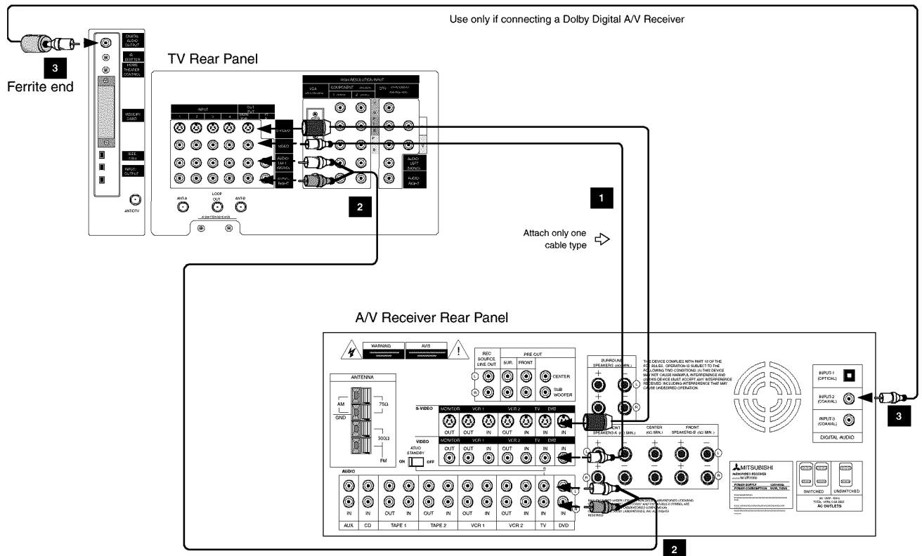
Figure 1. Connecting an Audio/Video Receiver
