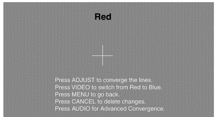
Figure 2. Convergence screen
