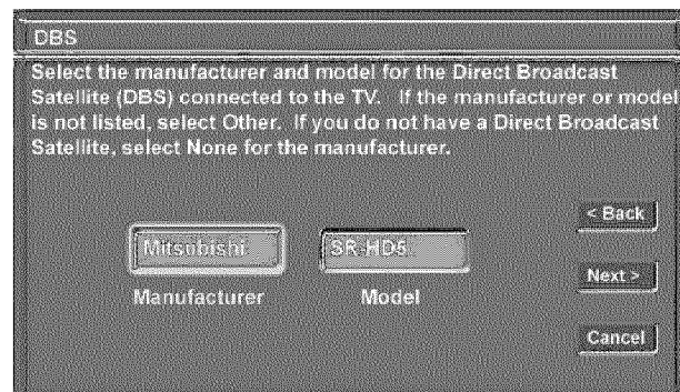
Figure 1. DBS menu.
