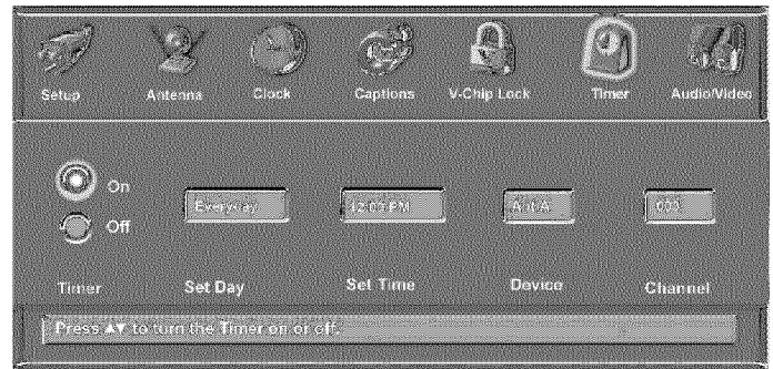
Figure 3. Timer menu
