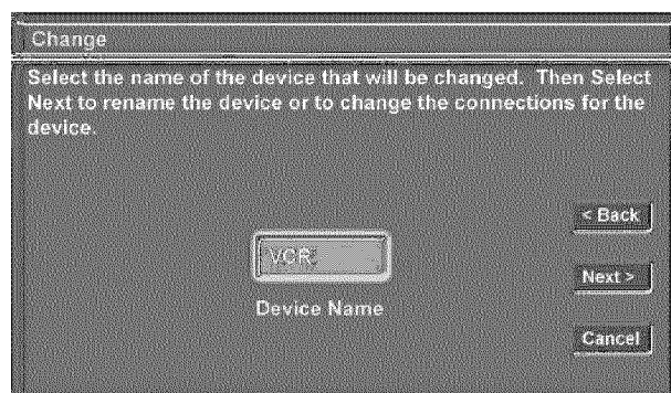
Figure 3. Change menu.
