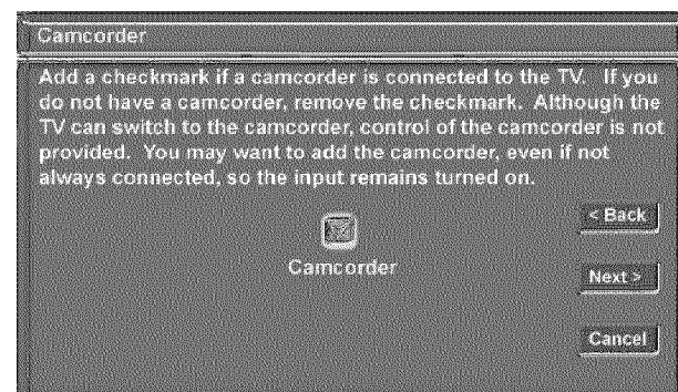
Figure 3. Camcorder menu.
