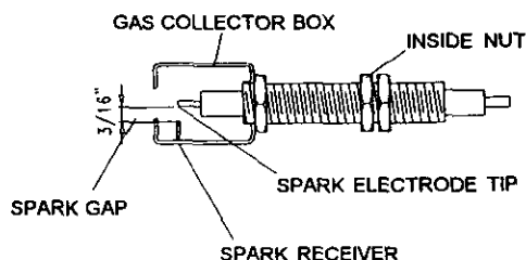
Figure 11 - Side View
