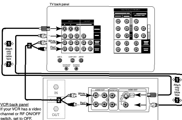
Figure 3. Connecting the VCR Audio/Video.
