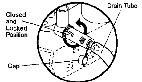
Oil Drain Valve
