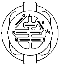
IGNITION SWITCH
