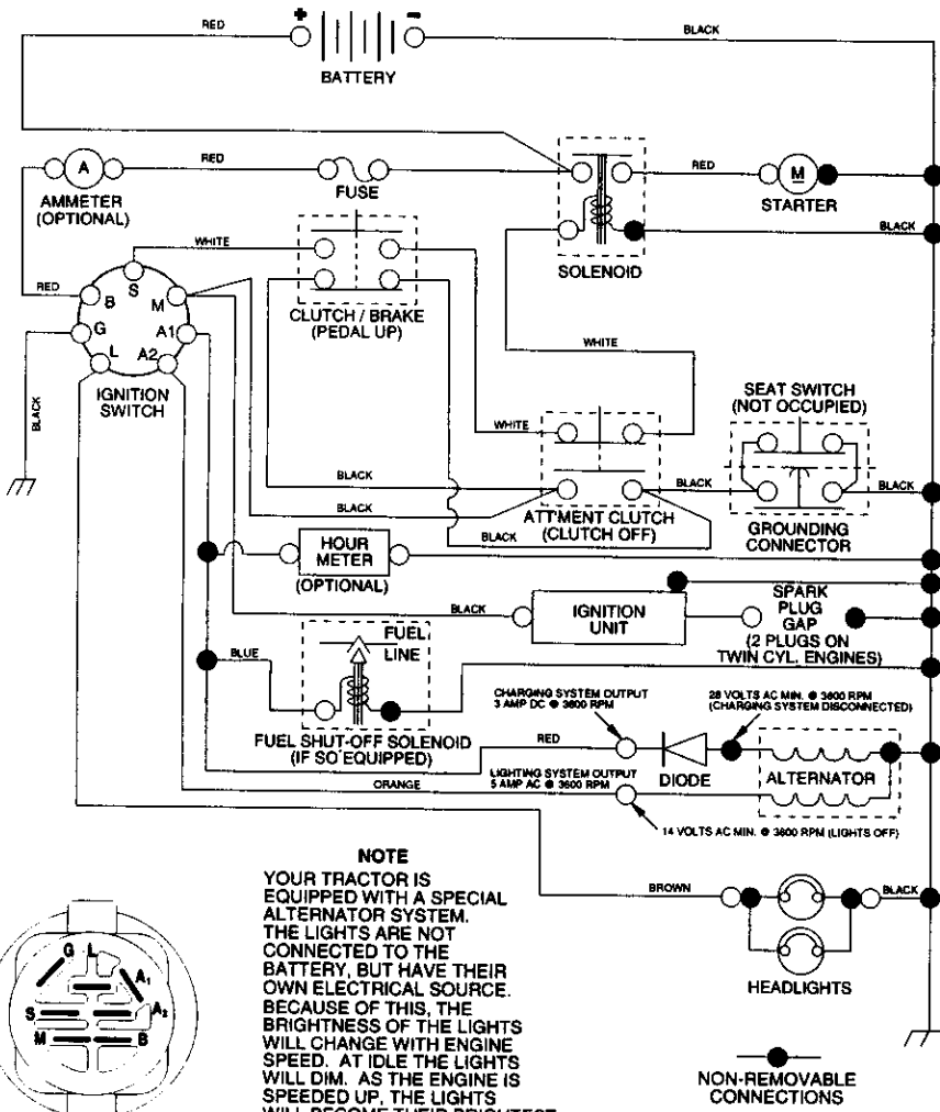
IGNITION SWITCH
