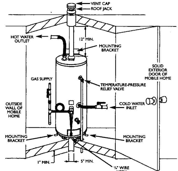
INSTALLATION IN ENCLOSURE OF MOBILE HOME WITH SOLID EXTERIOR DOOR
