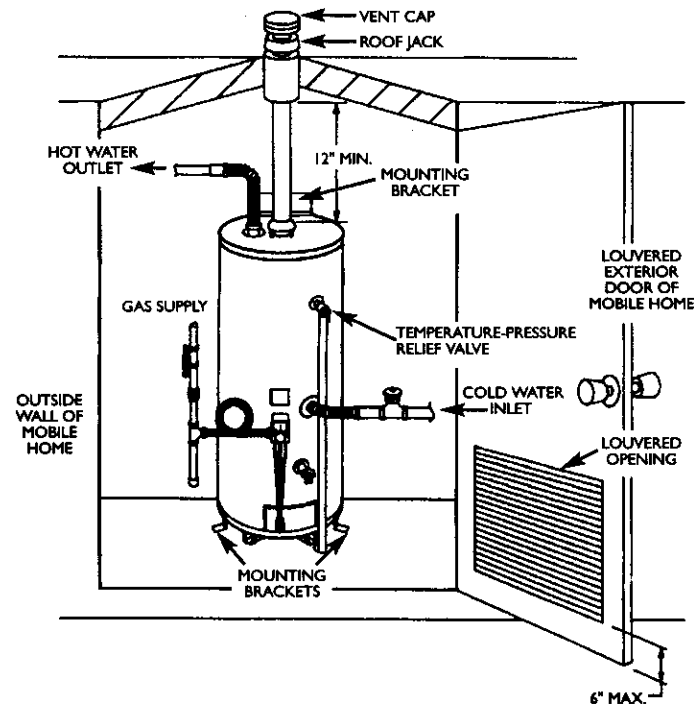
INSTALLATION IN ENCLOSURE OF MOBILE HOME WITH LOUVERED EXTERIOR DOOR
