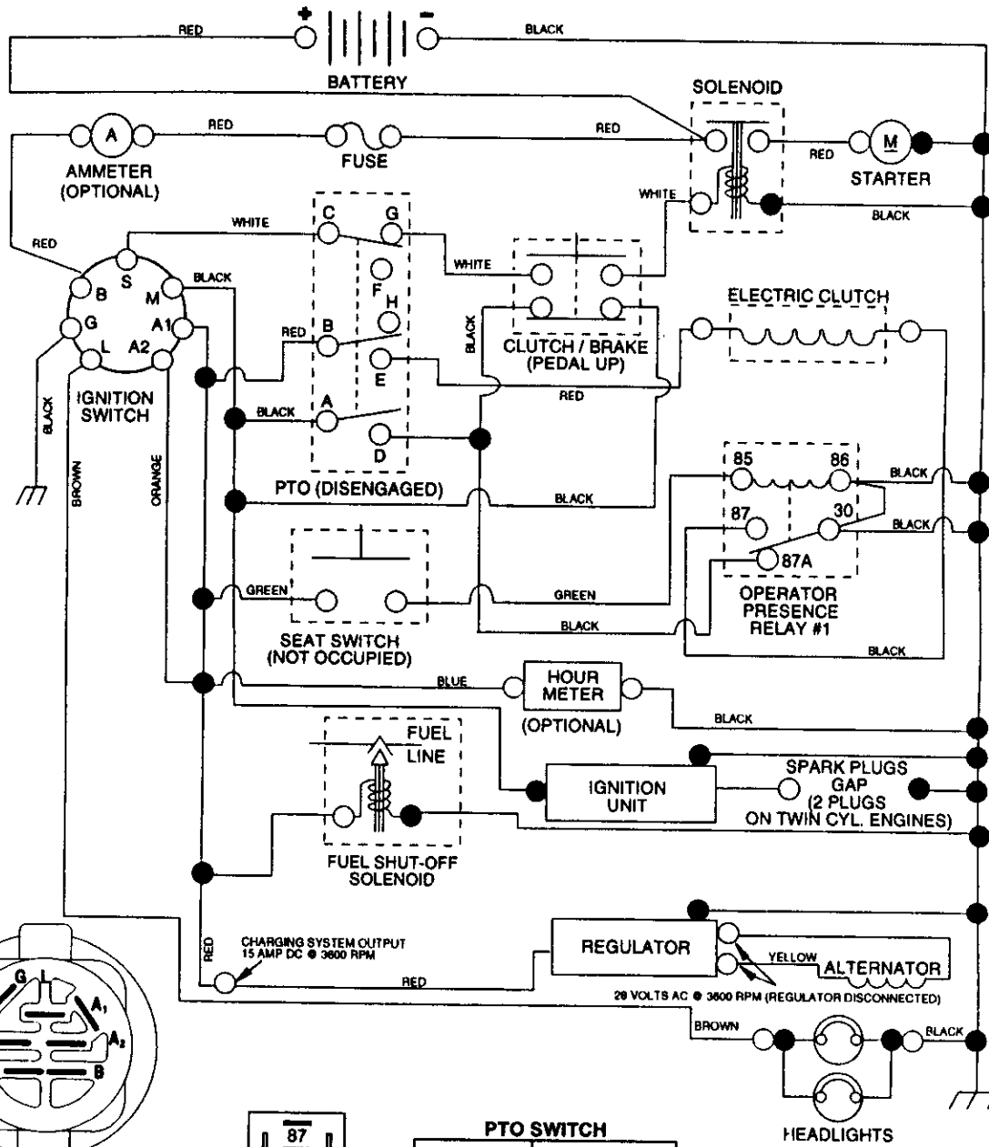
IGNITION SWITCH
