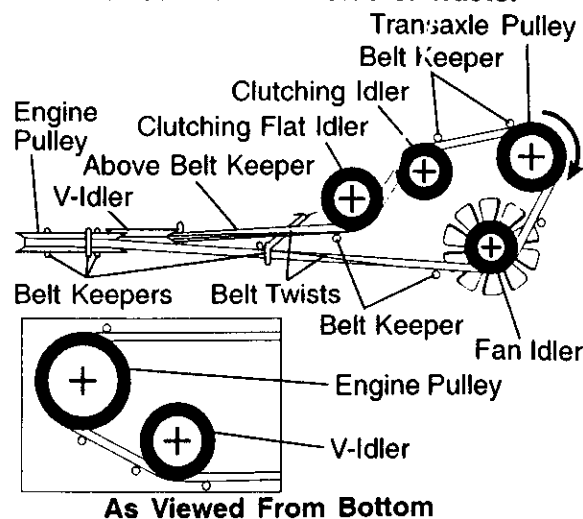
Tractor V-Belt Drive Schematic Viewed From L.H. Side of Tractor
