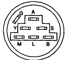
IGNITION SWITCH
