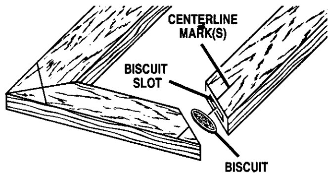
FLAT MITER JOINTS Fig. 16
