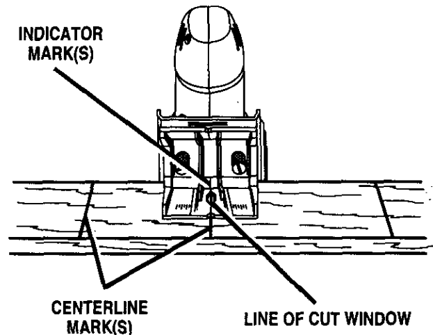
TOP VIEW OF DETAIL BISCUIT JOINER Fig. 7
