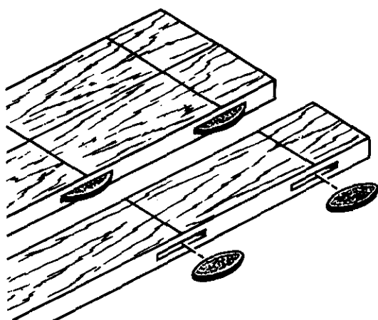
EDGE-TO-EDGE JOINTS
