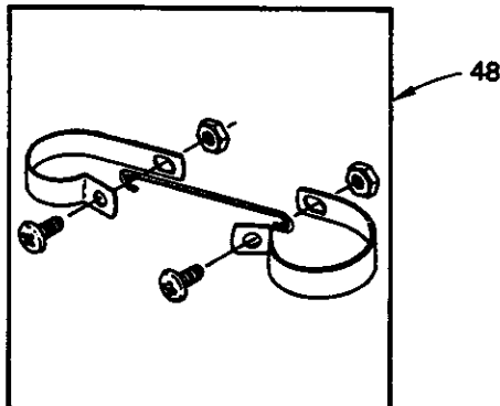
INLET - OUTLET GROUNDING CLAMPS
