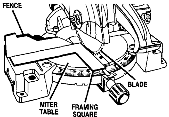
VIEW OF BLADE NOT SQUARE WITH FENCE, ADJUSTMENTS ARE REQUIRED Fig. 18
