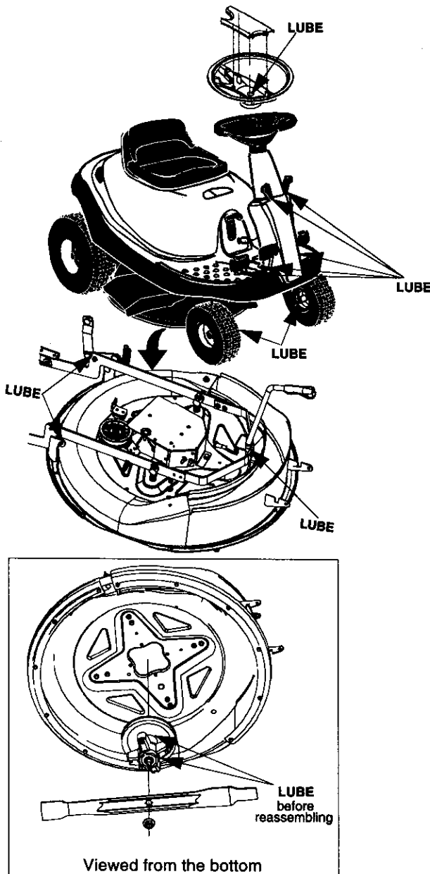
Figure 27: Lubrication Chart
