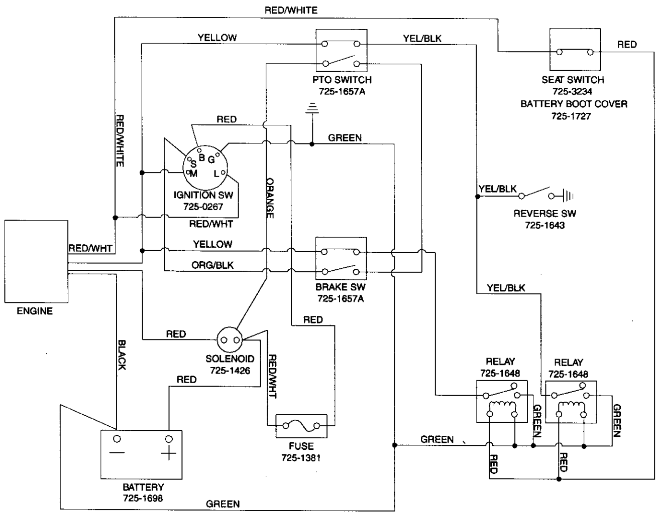
COMPLETE WIRE HARNESS (629-0902)
