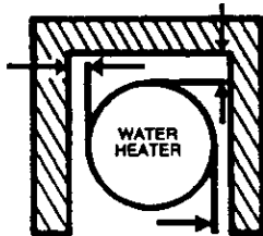
ALCOVE INSTALLATION (ACCEPTABLE)
