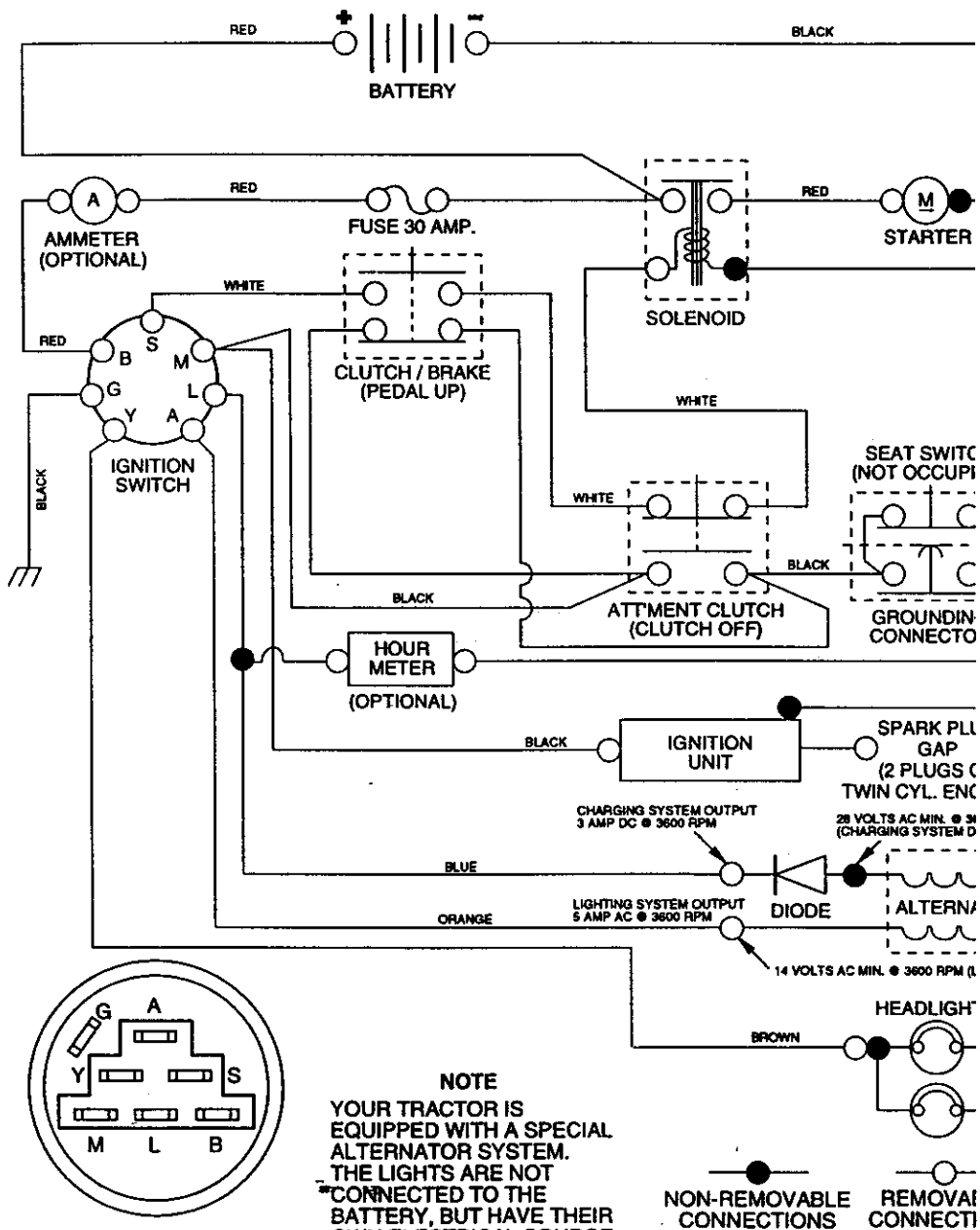
IGNITION SWITCH
