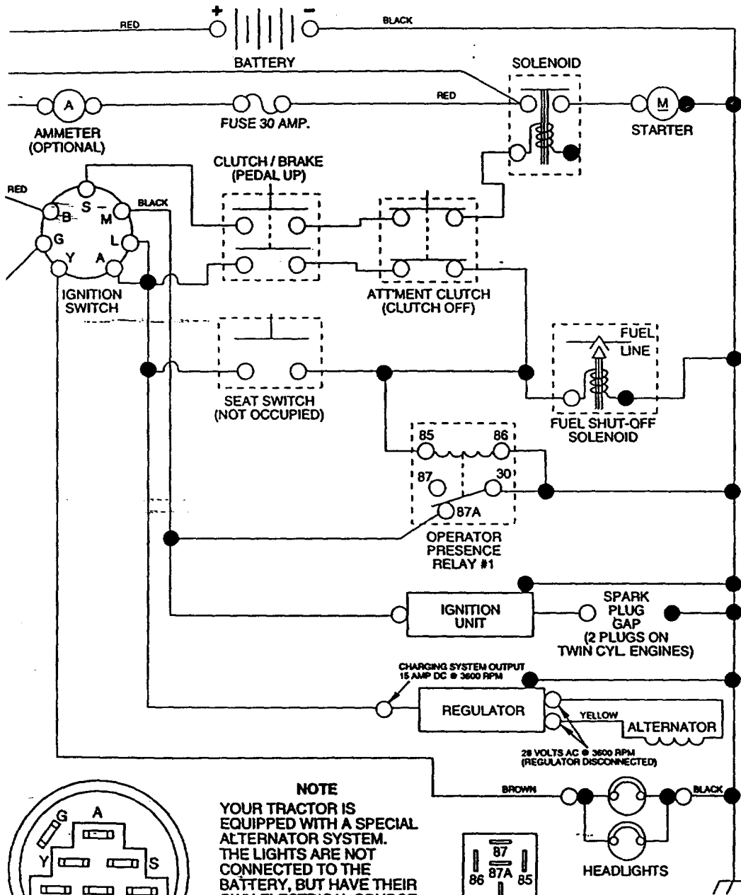
RELAY
