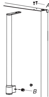
A. Flat-head handle screws B. Setscrew
