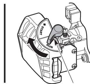
Choke Lever
