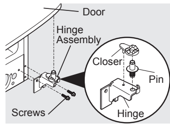
Adjustable Hinge
