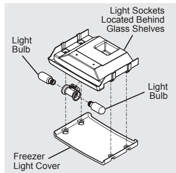
Freezer Light
