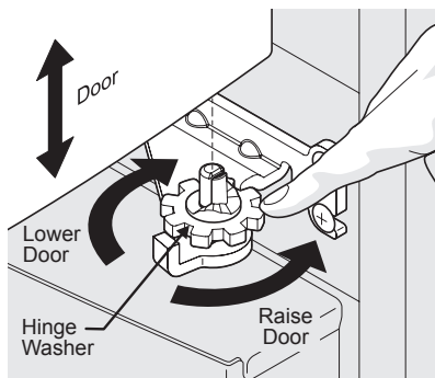
Raising/Lowering Door
