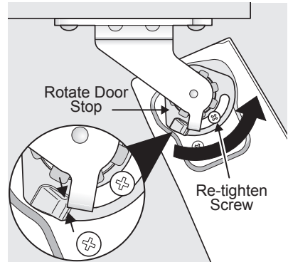
Re-tighten Screw
