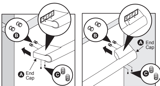
Mounting Freezer Handle
