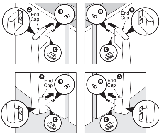
Mounting Refrigerator Handles
