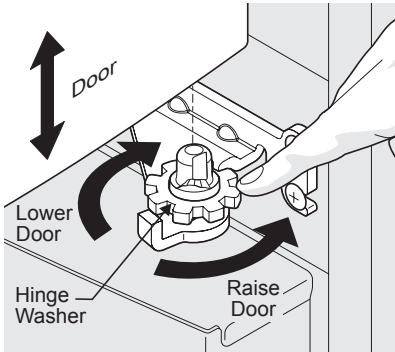
Raising/Lowering Door
