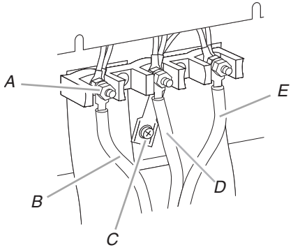
A. 10-32 hex nut D. Neutral (white) wire B. Line 1 (black) E. Line 2 (red) C. Ground-link screw
