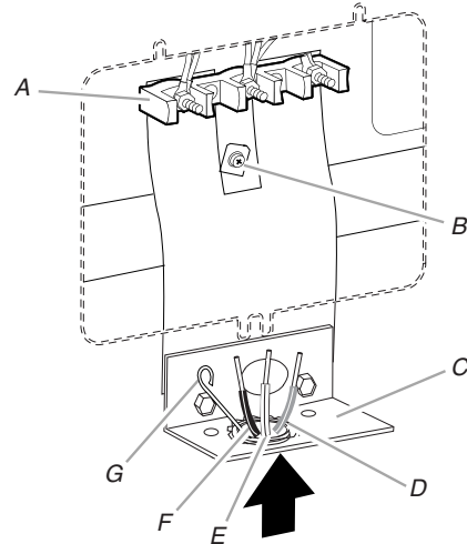
A. Terminal block E. Neutral (white) wire B. Ground-link screw F. Line 1 (black) wire C. Cord/conduit plate G. Bare (green) ground wire D. Line 2 (red) wire
