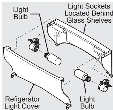
Refrigerator Light
