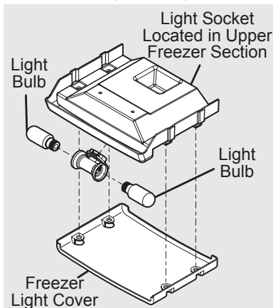
Freezer Light
