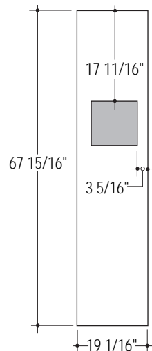
3/4" Thick Custom Panels with Standard Handles
