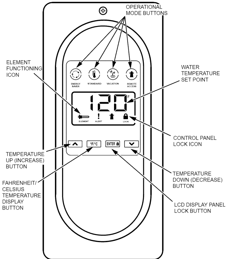
ENERGY SAVER MODULE (ESM)
