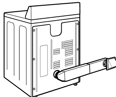
Periscope installation
