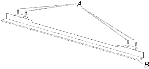
A. Phillips head screws (4) B. Warming drawer deflector (1)
