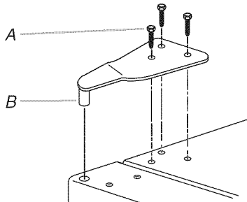
A. 5/16" Hex-head hinge screw B. Top hinge pin
