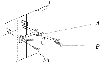
A. Center hinge B. 5/16" Hex-head hinge screw
