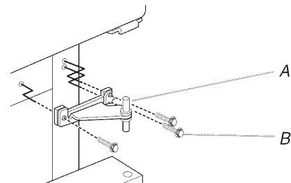
A. Center hinge B. 5/16" Hex-head hinge screws
