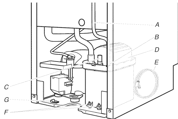
A. Vent tube B. 5/8" hose clamp C. Drain pump discharge tube D. Drain pump E. Ice maker unit power cord F. #8-32 x 3/8" pump mounting screws G. Drain pump power cord, clamp and screw
