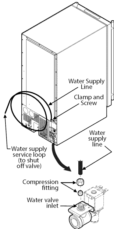
Figure 5 Back view of ice machine
