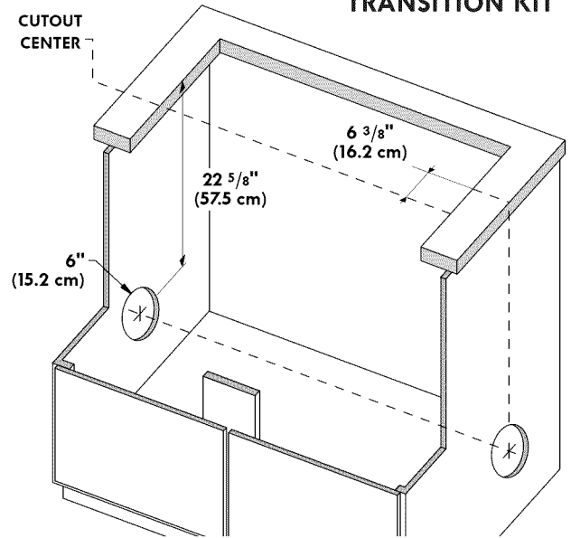
Figure 13A – 30" MODEL ALTERNATE DUCTWORK HOLE
