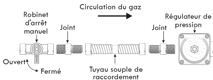
Figure 24 – RACCORDS DE GAZ
