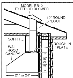
TYPICAL ROOF MOUNTED INSTALLATION
