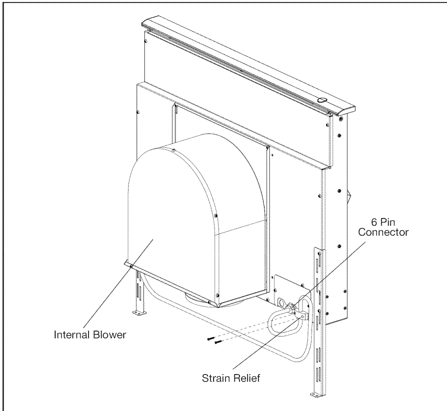
Fig. 9 – Internal Blower
