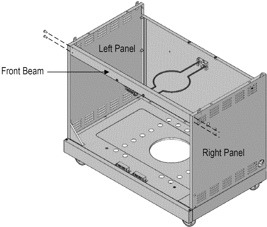
1/4-20 x 5/8" Screw Qty. 4
