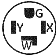
TYPICAL 30 AMP RECEPTACLE FOR DRYER
