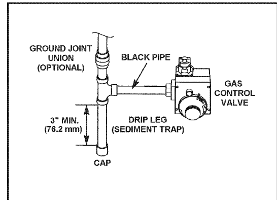
FIGURE 20. GAS PIPING WITH ALL BLACK IRON PIPE TO GAS CONTROL.
