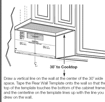
Plate position – beneath framed recessed cabinet bottom.
