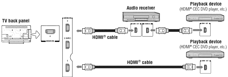
(Sample Illustration) L9400U Series—Connecting an HDMI® CEC compatible audio system and playback device
