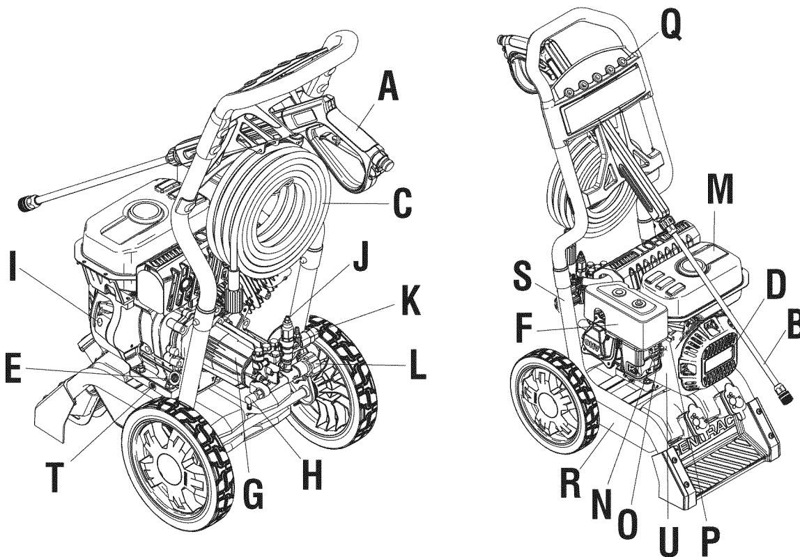
Figure 1 – Features & Controls
