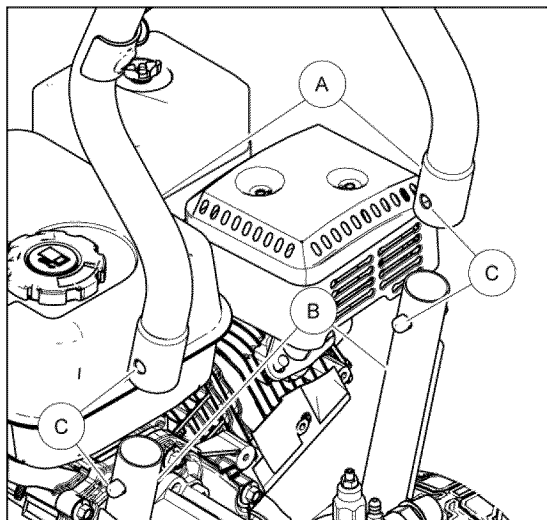
Figure 2 – Attach Handle
