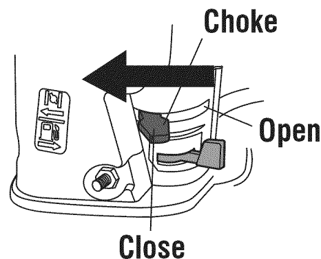
Figure 24 – Choke Lever
