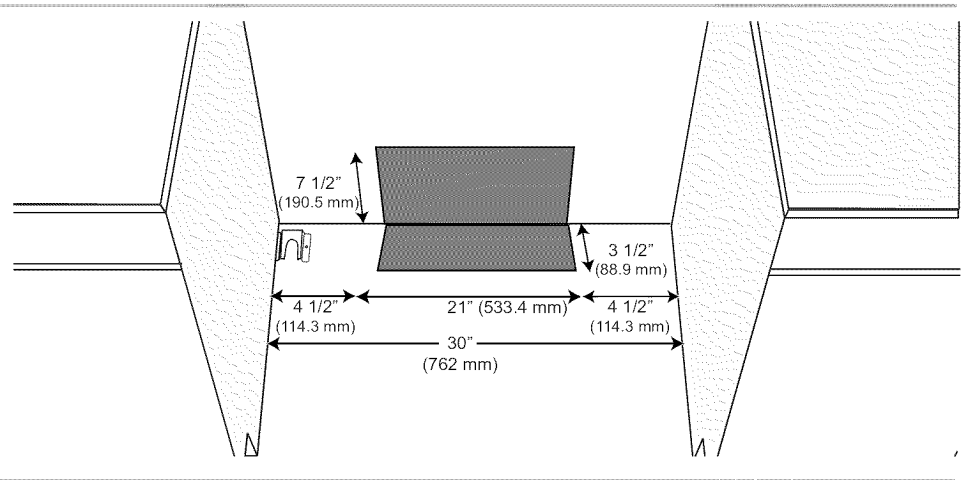
Figure 1: Cooktop Clearances
