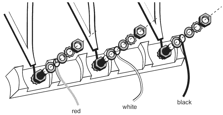
Figure 12: Four Wire Range Cord Connection (continued)
