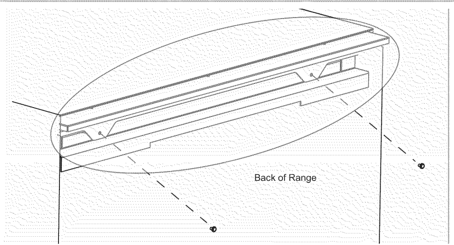
Figure 7: Install Backwall Trim Strip
