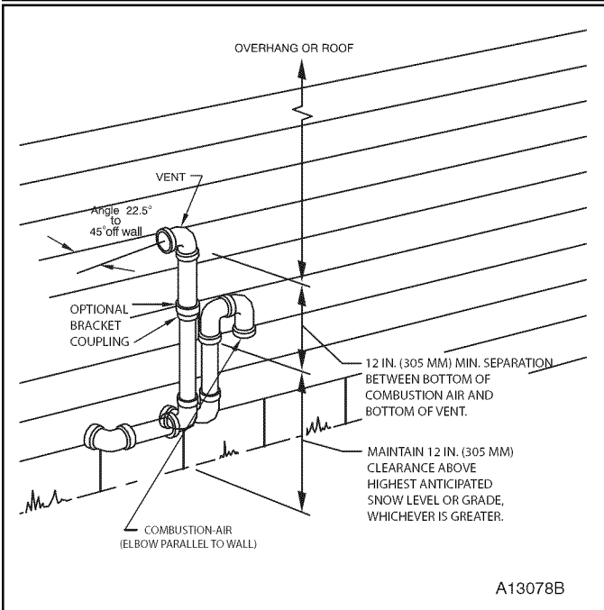
Figure 47 Combustion Air and Vent Pipe Termination for Direct Vent (2-Pipe) System
