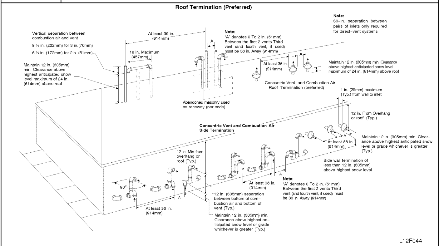
Figure 47 Combustion Air and Vent Pipe Termination for Direct Vent (2-Pipe) System
