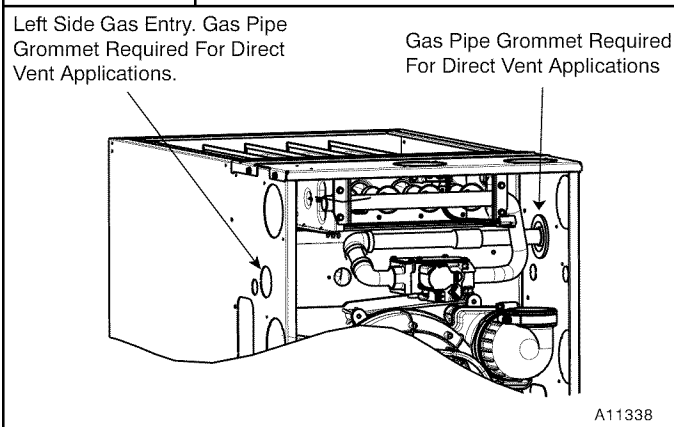
Figure 34 Gas Entry
