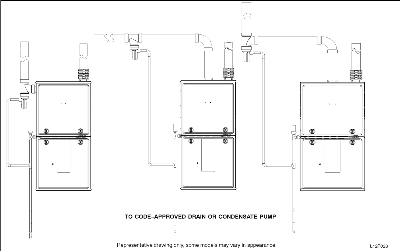
Figure 50 Optional Combustion Air Inlet Moisture Trap
