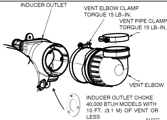
Figure 52 Upflow Configurations
