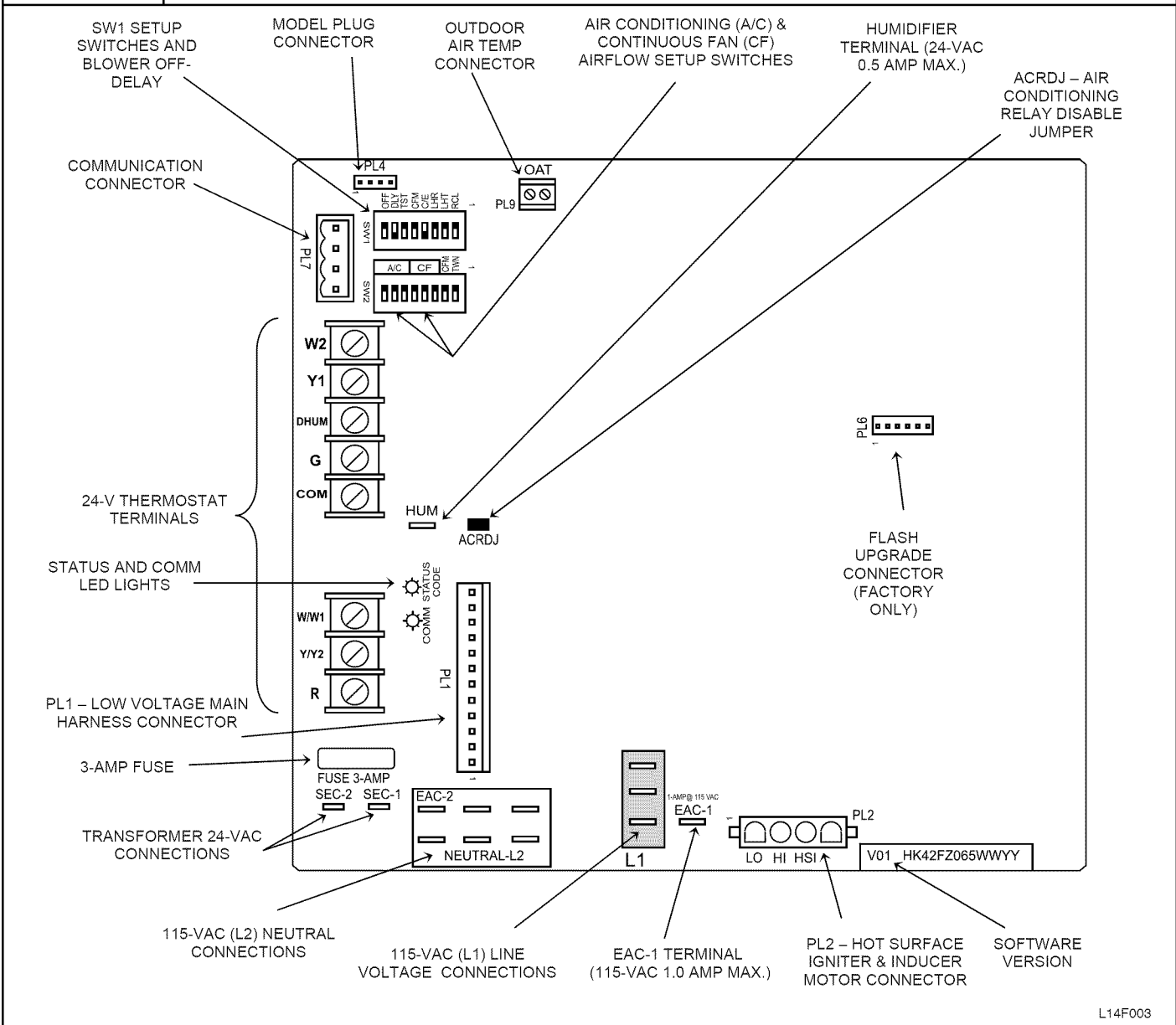
Figure 40 Example of Variable Speed Furnace Control for PWM Blower Motor
