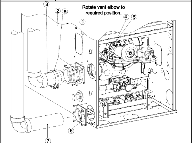
DOWNFLOW LEFT - VENT CONFIGURATION
