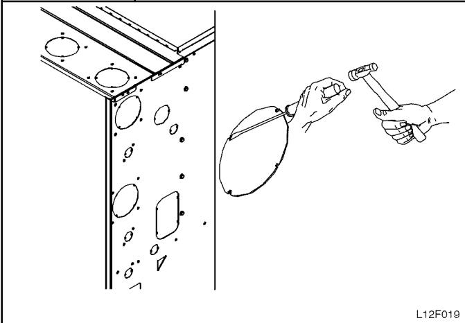
Figure 13 Knockout Removal
