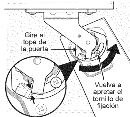
Re-tighten Set Screw
