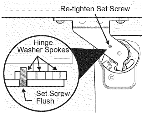
Set Screw (where applicable)
