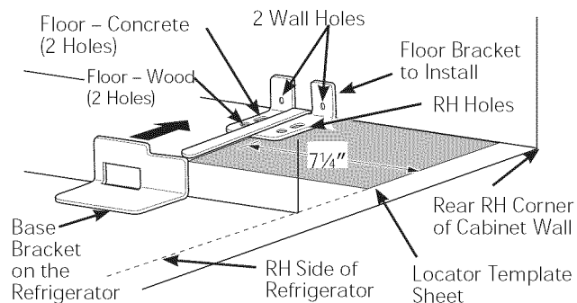
Figure 1 – Installation Overview
