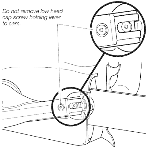
Figure 15 - Lever and Cam Screw Assembly Location
