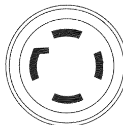
Fig 2-10: Tomacorriente de 120/240 VCA, 30 A
