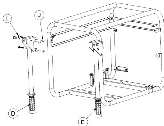
Figure 2 – Handle Kit
