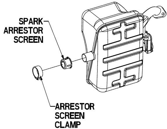
Figure 16 - Spark Arrestor
