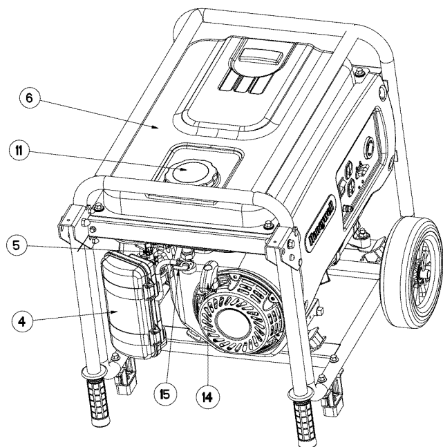
Figure 4 - Generator Controls
