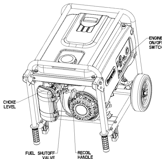
Figure 13 - Engine Controls
