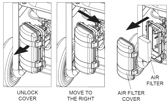
Figure 17 - Air Filter
