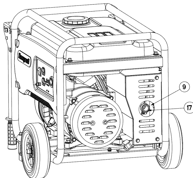
Figure 6 - Generator Controls
