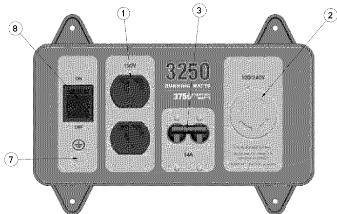
Figure 3 - Control Panel
